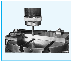
#240-0131 locating work from straight edge
