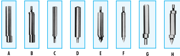
#240-0131 locating work from straight edge
